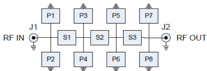
NETWORK SCHEMATIC
