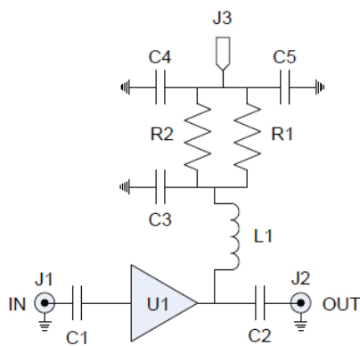
AMPLIFIER SCHEMATIC
